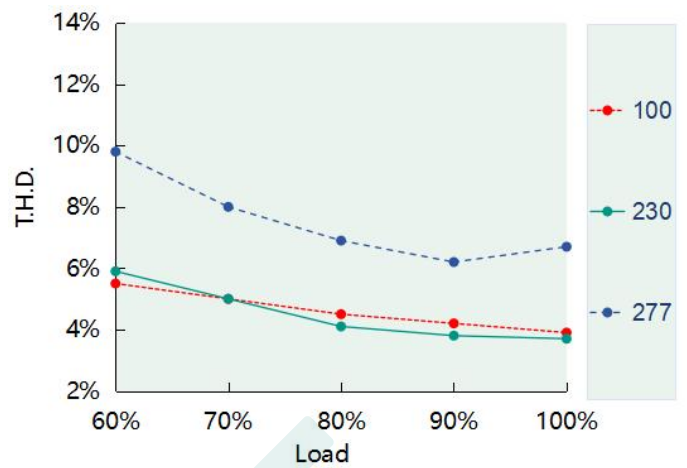
THD vs. Load ( DL-150Z-56A/P-MXL )
