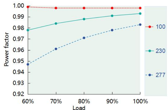
Power Factor vs. Load ( DL-150Z-107A/P-MXL )
