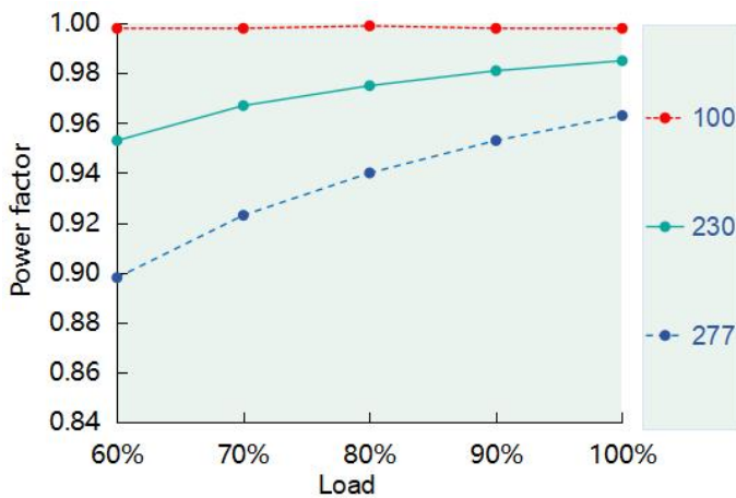
Power Factor vs. Load ( DL-150Z-214A/P-MXL )
