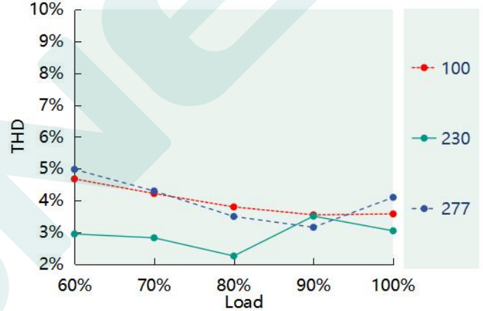
THD vs. Load ( DL-150Z-214A/P-MXL )
