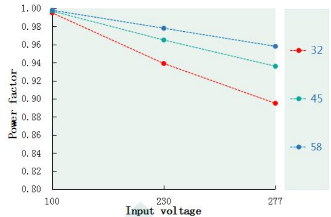
Power factor VS Input voltage(DL-20Z-MAL)
