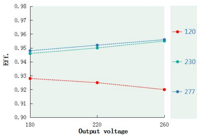
Eff. VS Output voltage DL-400W-V260X/T-PLS
