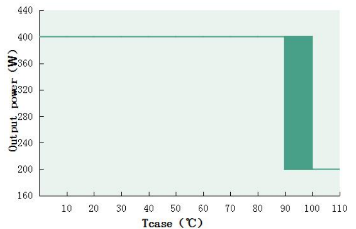
Output power VS Tcase(DL-400W-V260X/T-PLS)
