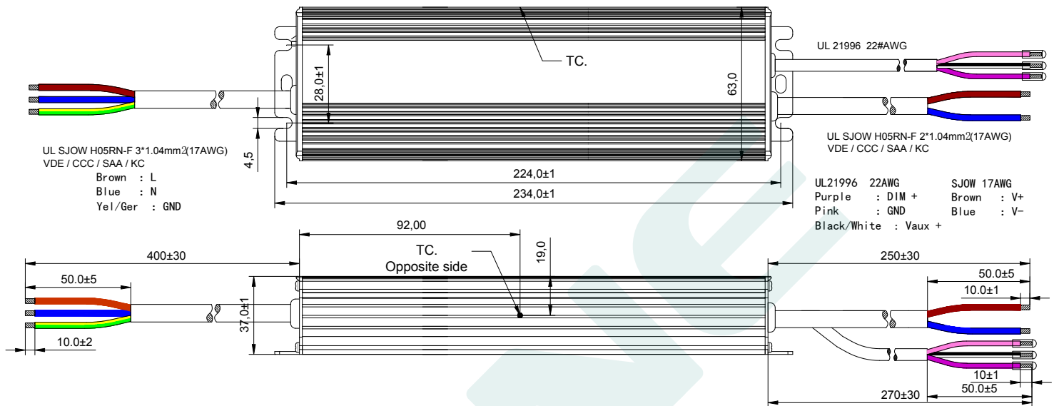
Dimension drawing DL-400W-V260X/T-PLS
