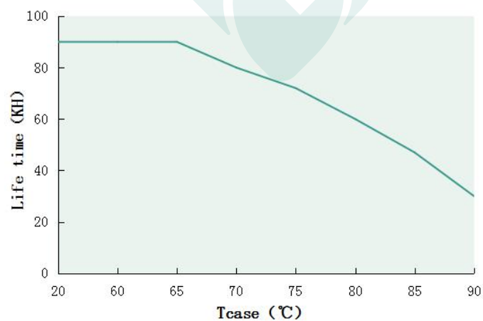
Tcase VS Lifetime(DL-400W-V260X/T-PLS)
