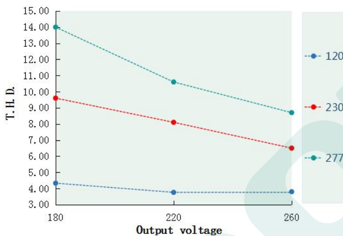
T.H.D VS Output power DL-400W-V260X/T-PLS
