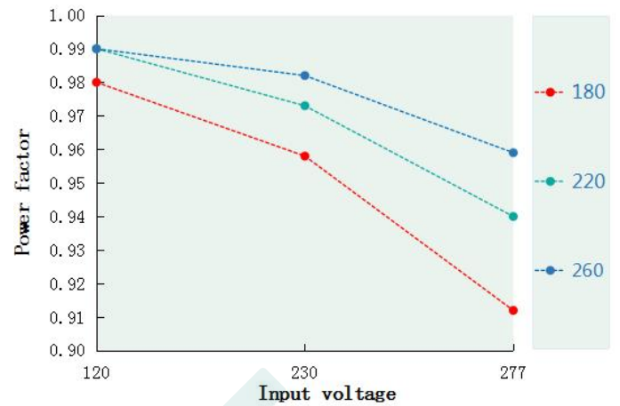
Power factor VS Input voltage DL-400W-V260X/T-PLS
