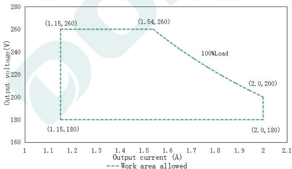
Output voltage VS output current of DL-400W-V260X/T-PLS (input: 120-277Vac)
