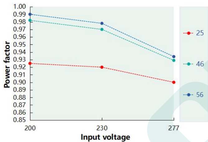
Power factor VS Input voltage(DL-200H-56A/P-MXC)
