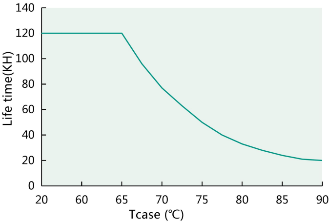
Tcase VS Lifetime(DL-200H-MXC)
