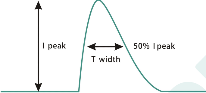
Inrush Current(DL-200H-MXC)
