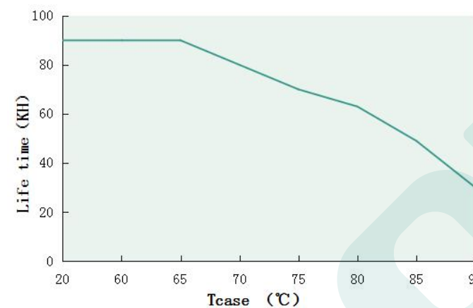
Tcase VS Lifetime(DL-960W-V260X-PLS)
