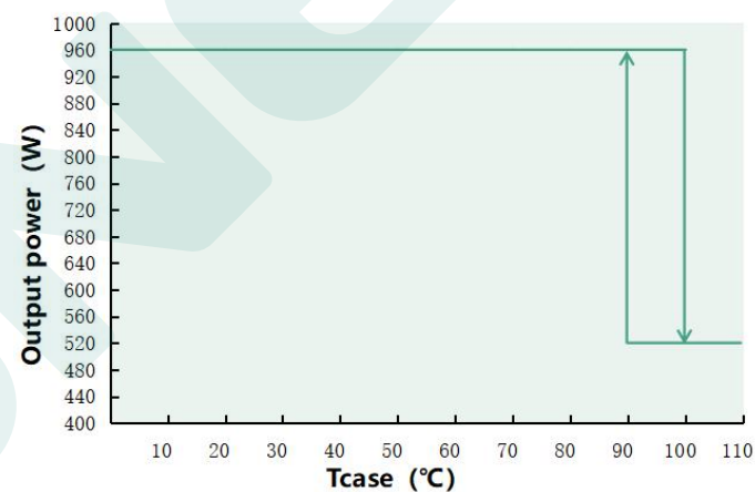
Output power VS Tcase(DL-960W-V260X-PLS)
