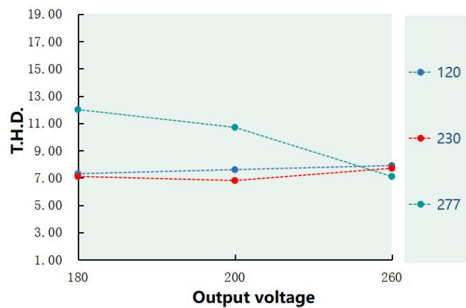
T.H.D VS Output voltage DL-960W-V260X-PLS
