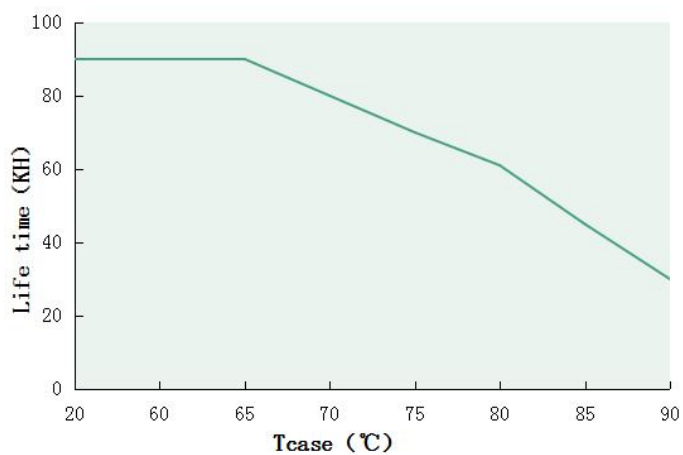
Tcase VS Lifetime(DL-240U-P-MUG)
