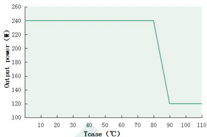
Output power VS Tcase (DL-240U-P-MUG)
