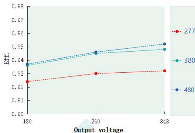
Eff. VS output voltage(DL-240U-343P-MUG)
