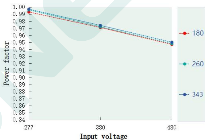
Power factor VS input voltage(DL-240U-343P-MUG)
