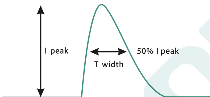
Inrush Current(DL-240U-P-MUG)
