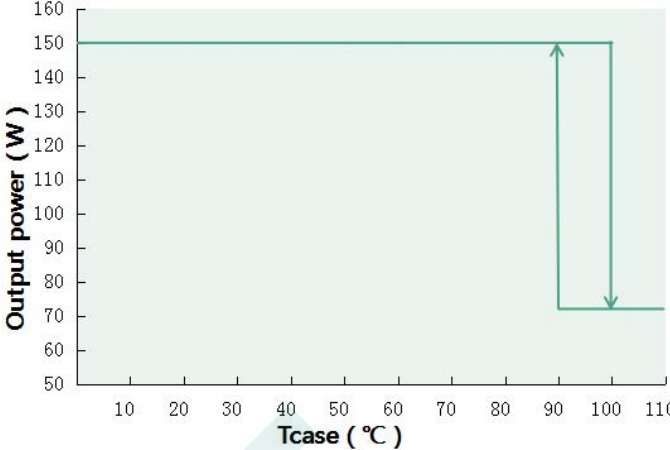
Output power VS Tcase (DL-150U-MUG)
