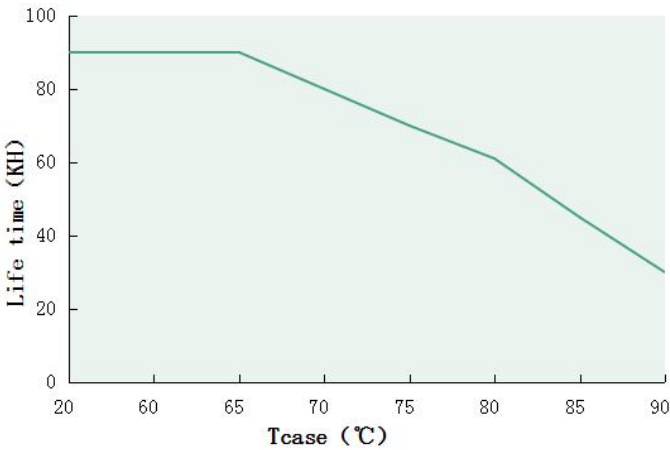
Tcase VS Lifetime(DL-150U-MUG)
