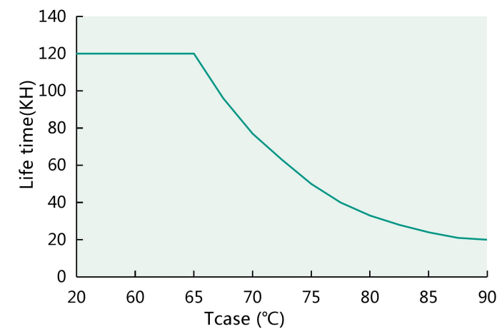
Tcase VS Lifetime(DL-240H-MXC)
