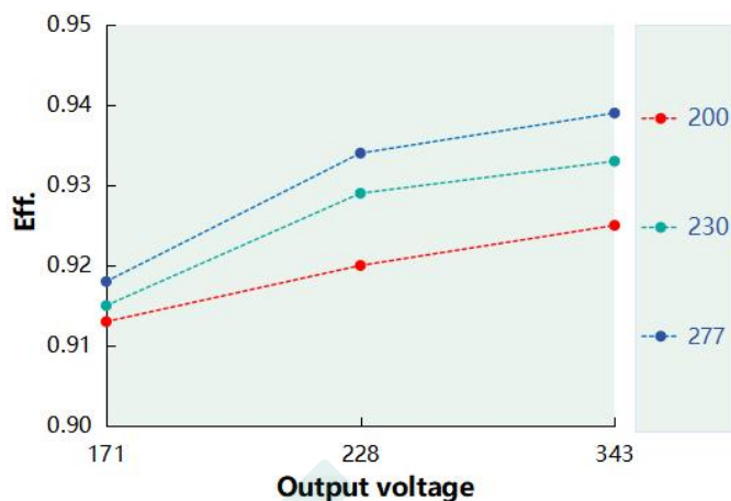
Eff. VS Output voltage(DL-240H-343P-MXC)
