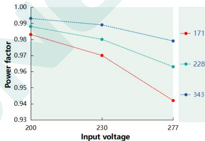
Power factor VS Input voltage(DL-240H-343P-MXC)
