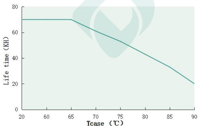
Lifetime VS Tcase ( DL-320Z-260X -PXS )
