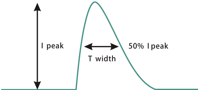
Inrush current(DL-80Z-260X -PXS)
