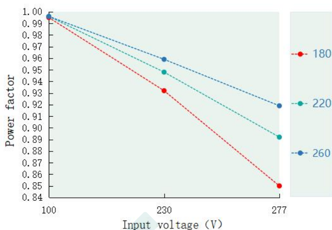
Power factor VS Input voltage(DL-80Z-260X-PXS)
