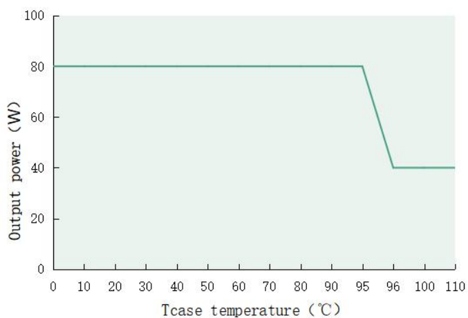
Output power VS Tcase temperature(DL-80Z-260X-PXS)
