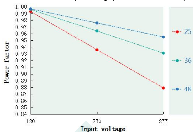
Power factor VS Input voltage(DL-50W-V48S/X-MTG)
