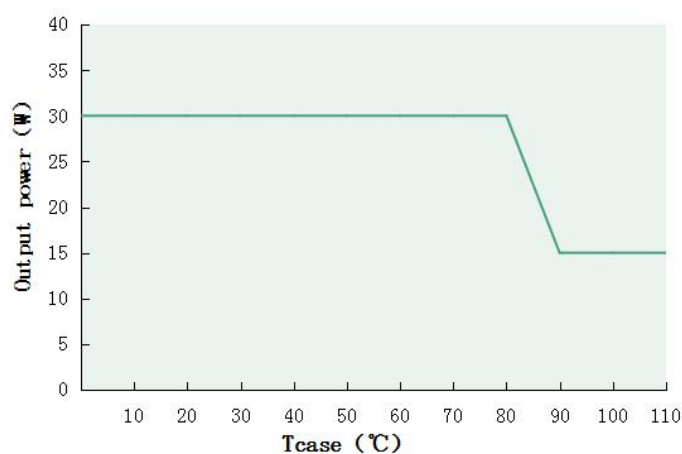
Output power VS Tcase (DL-50W-S/X-MTG)
