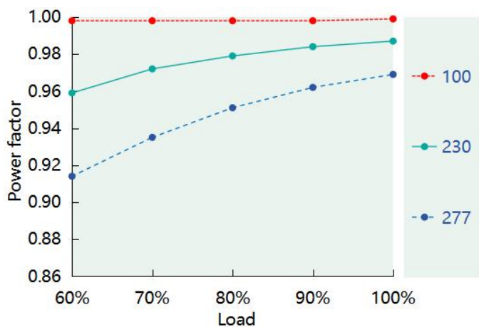
Power Factor vs. Load (DL-100Z-143A/P-MXL)
