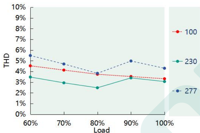
THD vs. Load ( DL-150Z-107A/P-MXL )
