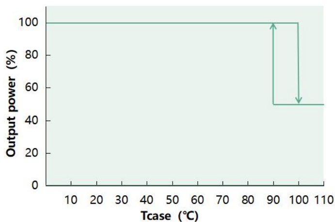
Output power vs. Tcase ( DL-150Z-MXL )
