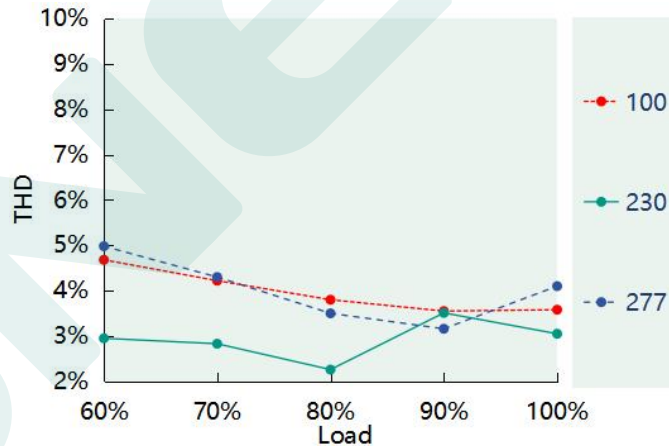
THD vs. Load ( DL-150Z-214A/P-MXL )
