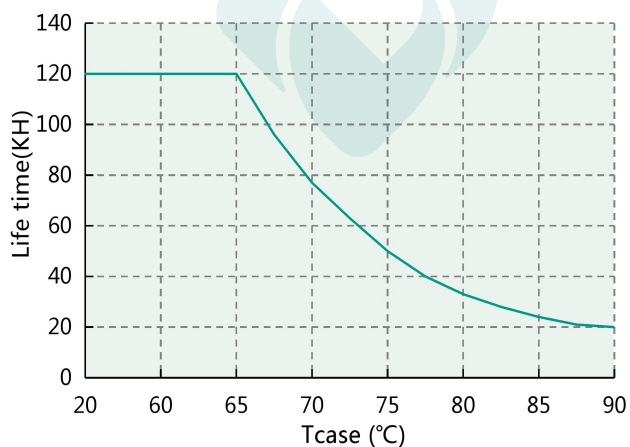
Lifetime vs. Tcase ( DL-150Z-MXL )
