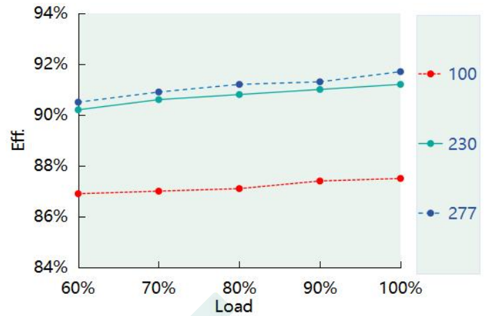
Eff. vs. Load ( DL-150Z-56A/P-MXL ) ( Io=2.68A )
