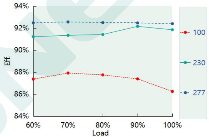
Eff. vs. Load ( DL-150Z-214A/P-MXL ) ( Io=0.7A )
