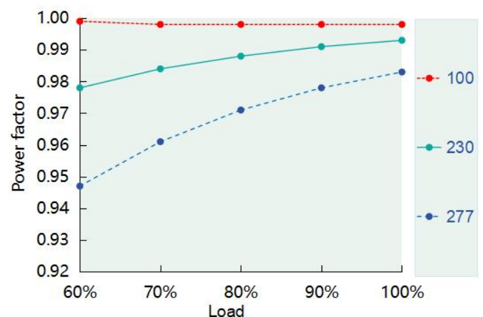
Power Factor vs. Load ( DL-150Z-107A/P-MXL )
