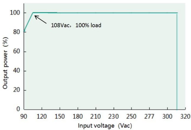
Output power vs. Input voltage ( DL-150Z-MXL )
