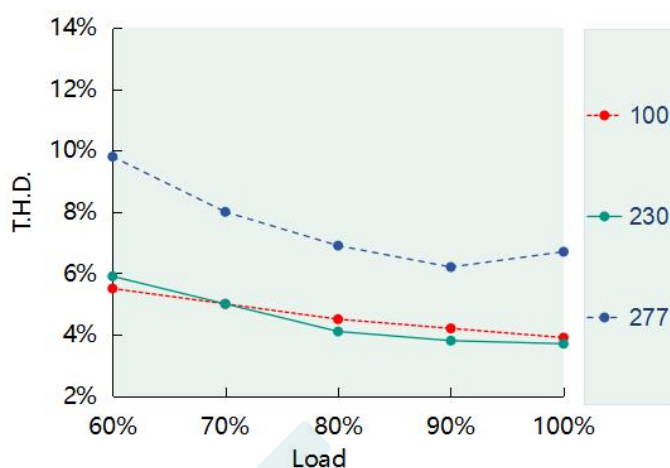
THD vs. Load ( DL-150Z-56A/P-MXL )
