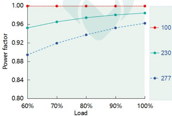
Power Factor vs. Load ( DL-150Z-56A/P-MXL )
