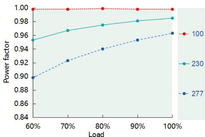
Power Factor vs. Load ( DL-150Z-214A/P-MXL )
