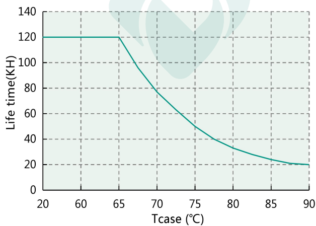
Tcase vs. Lifetime ( DL-100Z-MXL )
