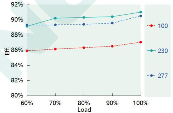
Eff. vs. Load ( DL-100Z-143A/P-MXL ) ( I_o=0.7A )
