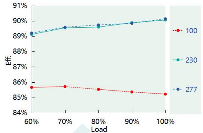
Eff. vs. Load ( DL-100Z-56A/P-MXL ) ( I_o=1.79A )
