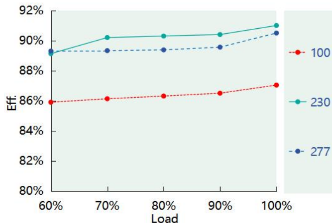
Eff. vs. Load ( DL-100Z-143A/P-MXL ) ( Io=0.7A )
