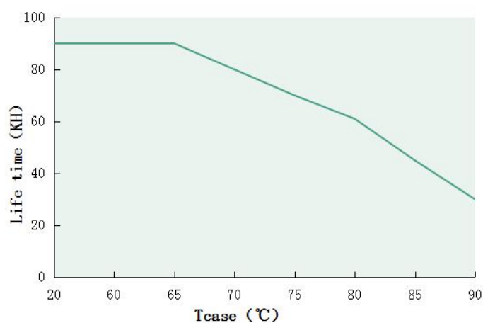
T case VS Lifetime(DL-100W-V48S/X-MTG)
