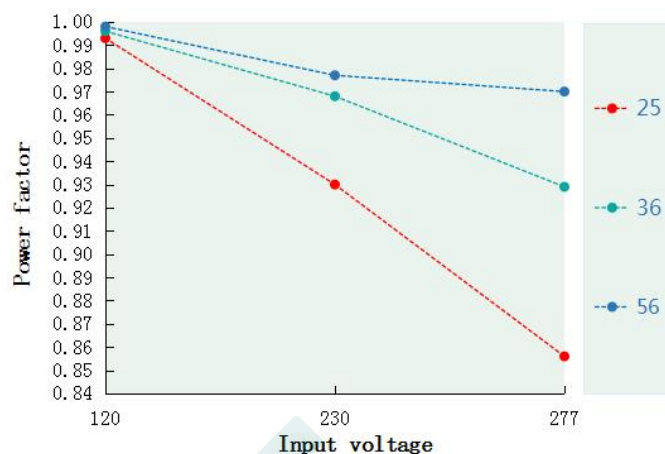
Power factor VS Input voltage(DL-100W-V48S/X-MTG)
