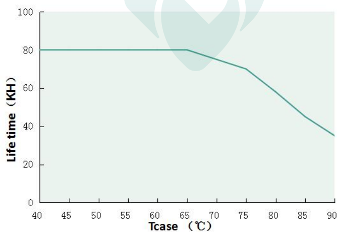
Lifetime VS Tcase ( DL-120V-260A/S/X-PXG )
