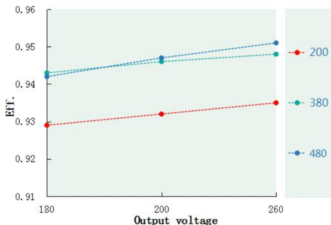
Eff. VS Output voltage ( DL-120V-260A/S/X-PXG )
