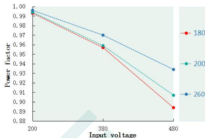
Power Factor VS Input Voltage ( DL-120V-260A/S/X-PXG )
