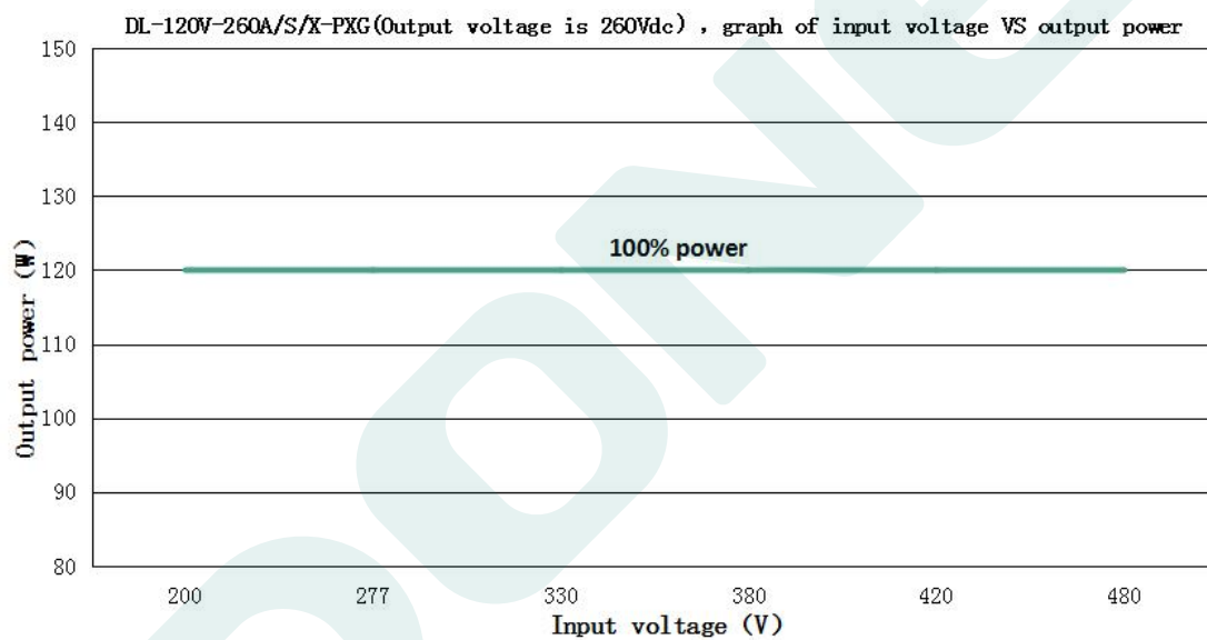
DL-120V-260A/S/X-PXG Input voltage VS Output Current( V_o=260V_{dc} ) VS Output Power
