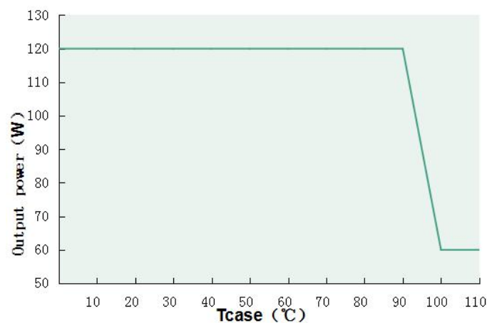
Output power VS Tcase ( DL-120V-260A/S/X-PXG )
