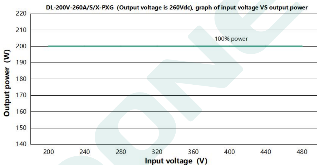
DL-200V-260A/S/X -PXG Input voltage VS Output Current( V_o=260V_{dc} ) VS Output Power
