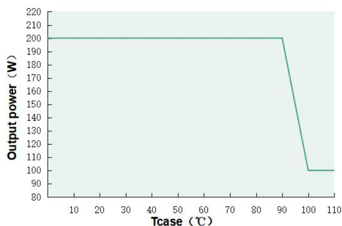
Output power VS Tcase ( DL-200V-260A/S/X-PXG )
