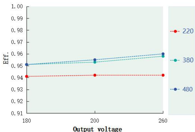
Eff. VS Output voltage ( DL-200V-260A/S/X-PXG )
