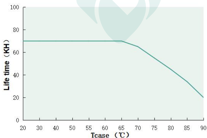
Lifetime VS Tcase ( DL-200V-260A/S/X-PXG )
