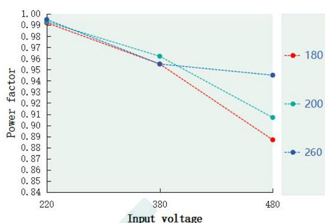
Power Factor VS Input Voltage ( DL-200V-260A/S/X-PXG )
