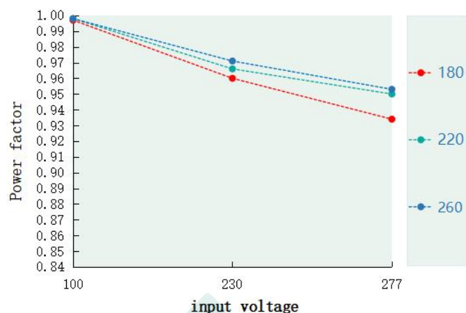
Power Factor VS Input Voltage (DL-80Z-260A/S/X-PXG)
