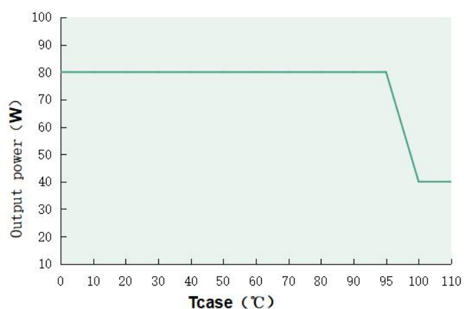
Output power VS Tcase (DL-80Z-260A/S/X-PXG)
