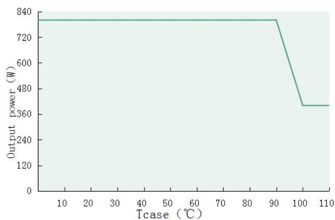
Output power VS Tcase DL-800V-260X/J-PXS
