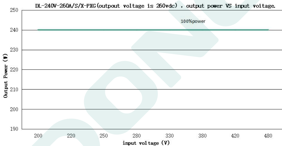
DL-240V-260A/S/X-PXG Input voltage VS Output Current( V_o=260Vdc ) VS Output Power
