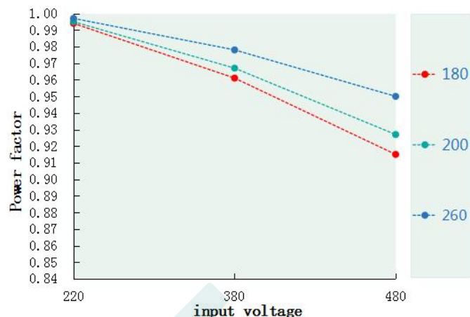
Power Factor VS Input Voltage ( DL-240V-260A/S/X -PXG )
