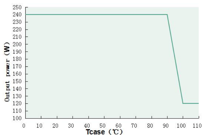
Output power VS Tcase ( DL-240V-260A/S/X -PXG )
