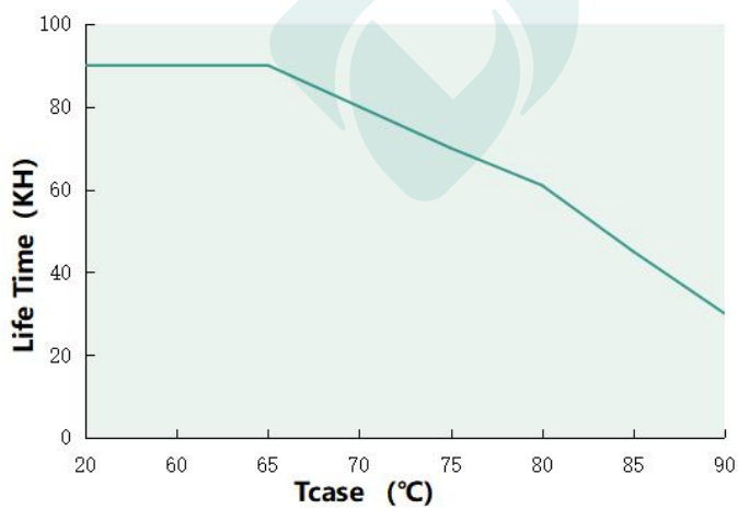
Tcase VS Lifetime DL-1000V-400X-PXS
