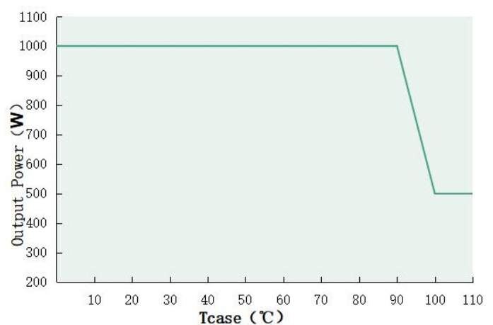
Output power VS Tcase DL-1000V-400X-PXS
