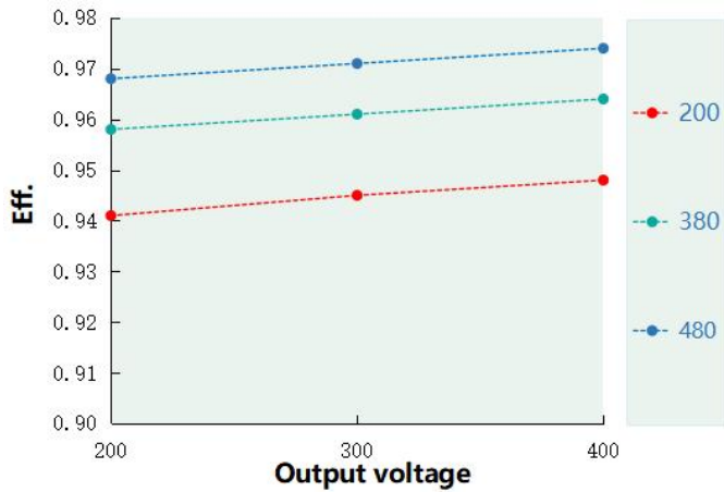
Eff. VS Output voltage DL-1000V-400X-PXS
