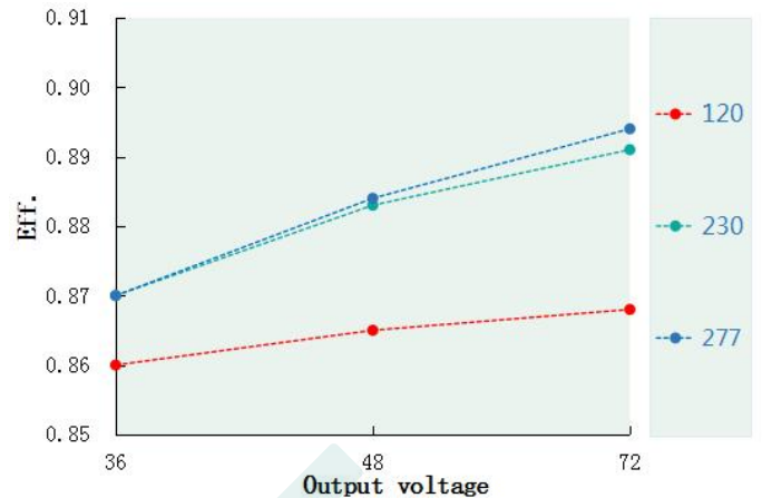
Eff. VS Output voltage(DL-50W-V72DX-MXG)
