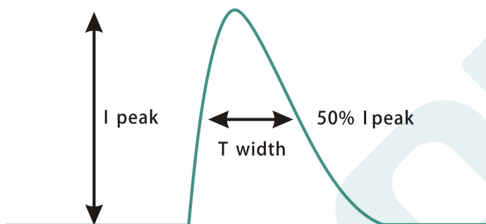
Inrush current(DL-50W-DX-MXG)
