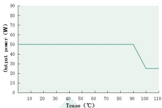
Output power VS Tcase (DL-50W-DX-MXG)
