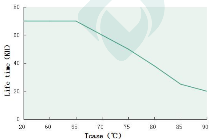
Tcase VS Lifetime(DL-50Z-MAL)
