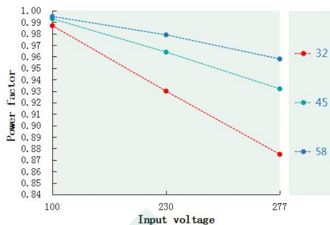
Power factor VS Input voltage(DL-50Z-MAL)
