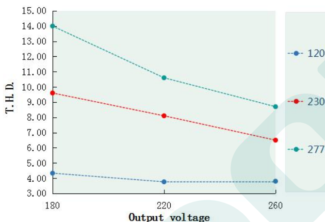
T.H.D VS Output power DL-400W-V260X/T-PLS
