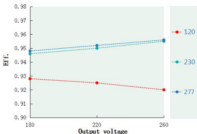
Eff. VS Output voltage DL-400W-V260X/T-PLS
