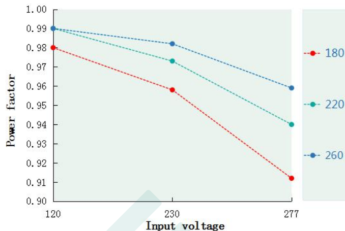
Power factor VS Input voltage DL-400W-V260X/T-PLS
