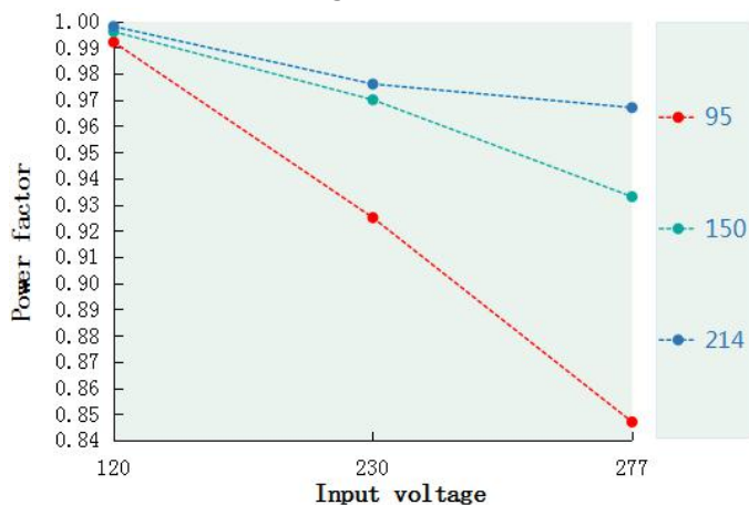
PF VS Input voltage(DL-150W-V214A/P/X-MDK)
