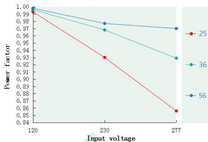
PF VS Input voltage(DL-150W-V56A/P/X-MDK)
