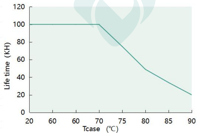
Tcase vs. Lifetime (DL-100Z-MXL)
