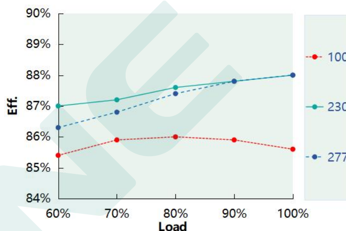
Eff. vs. Load
