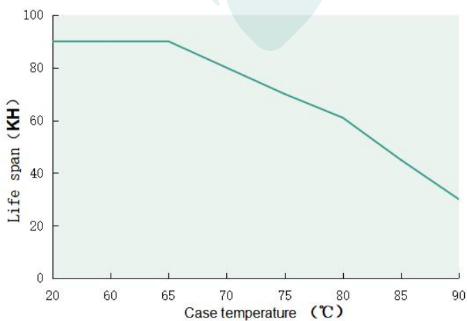
Tcase VS Lifetime(DL-40H-MXC)
